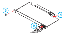
2-9 显卡安装
