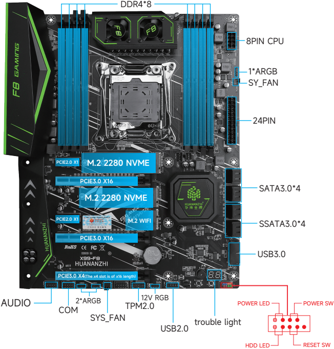
1-1 X99-F8 Motherboard Illustration
