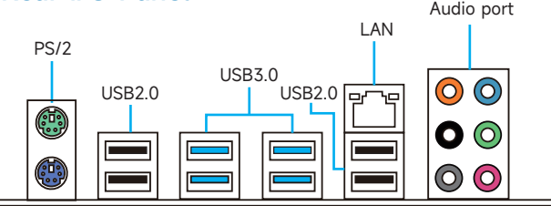
1-2 Overall Rear I/O Panel Display
